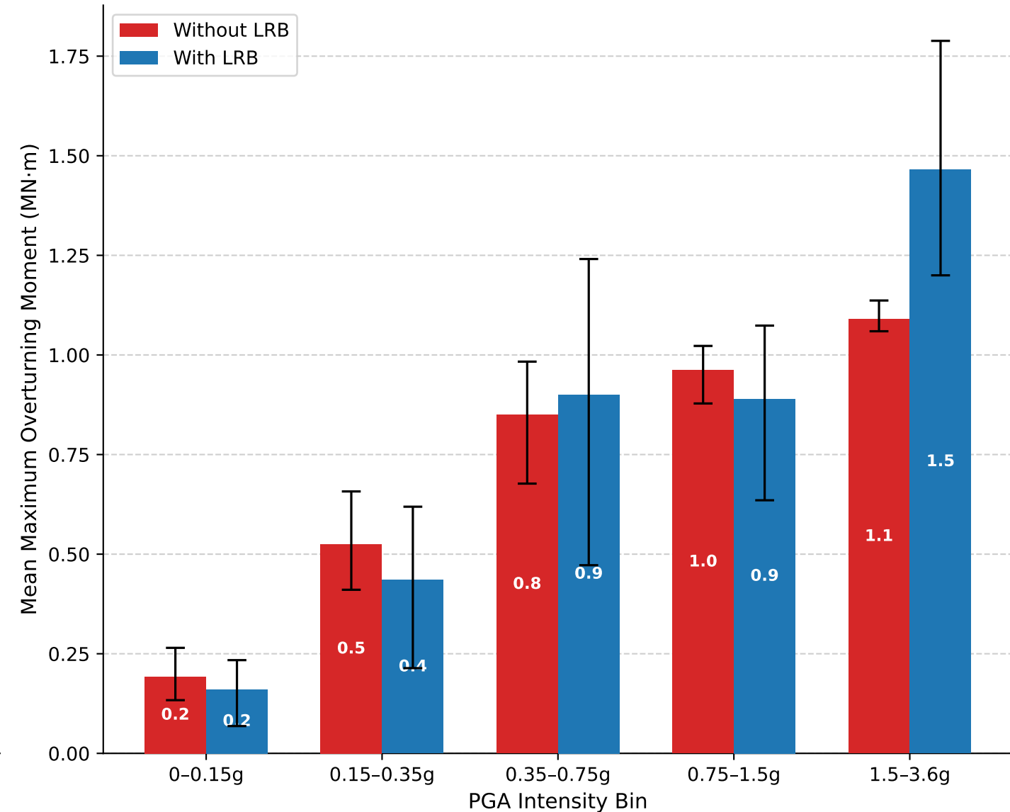
Maximum Overturning Moment
