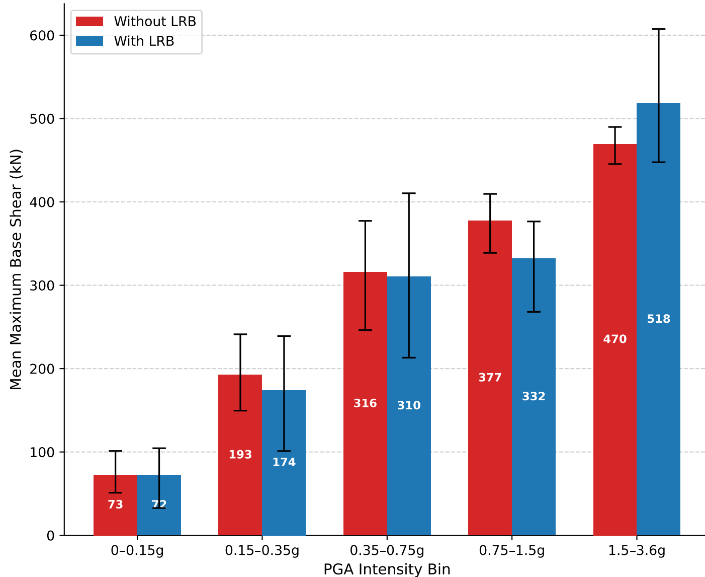
Maximum Base Shear
