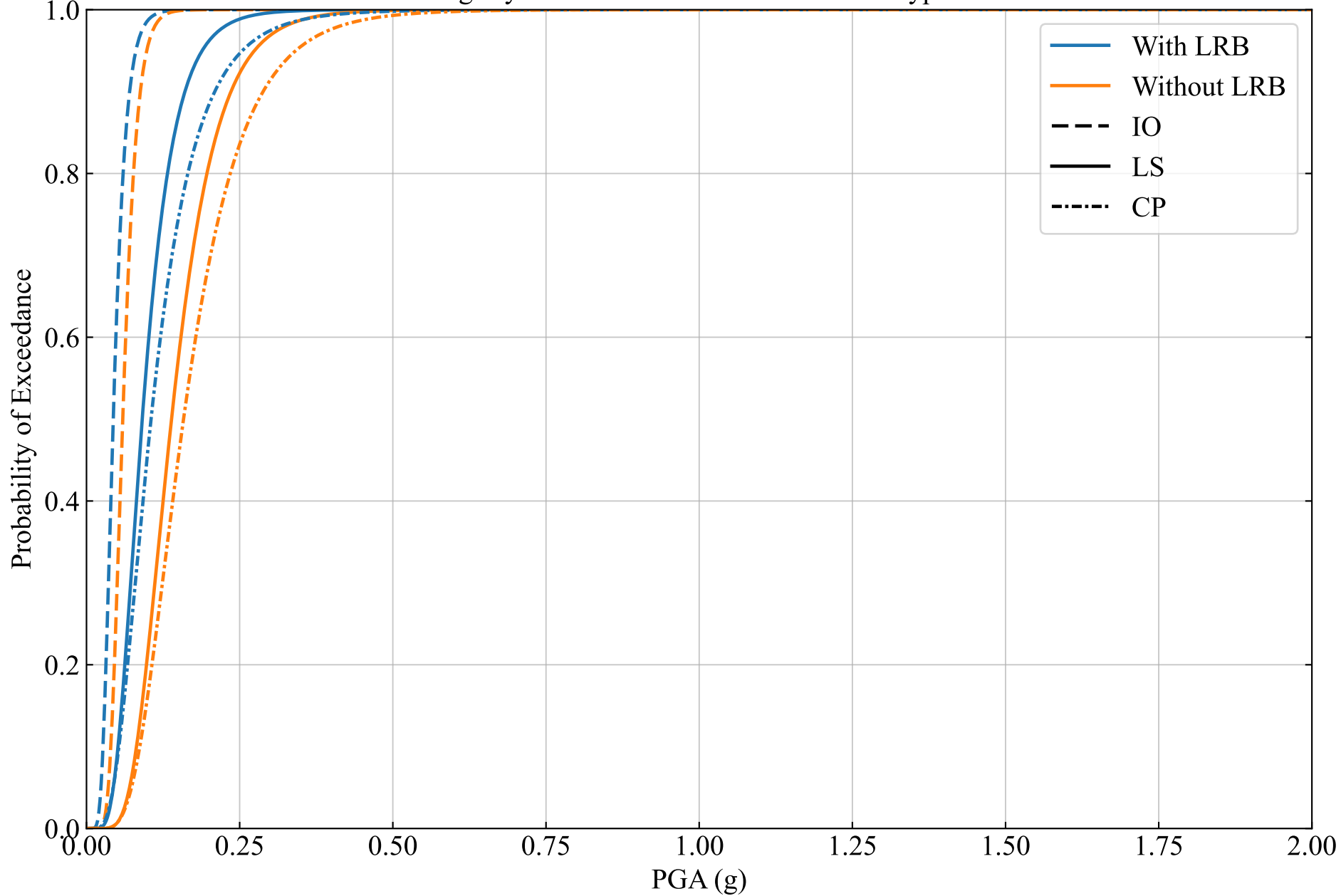
Fragility Curves for 100 kL Tank on Soil Type D
