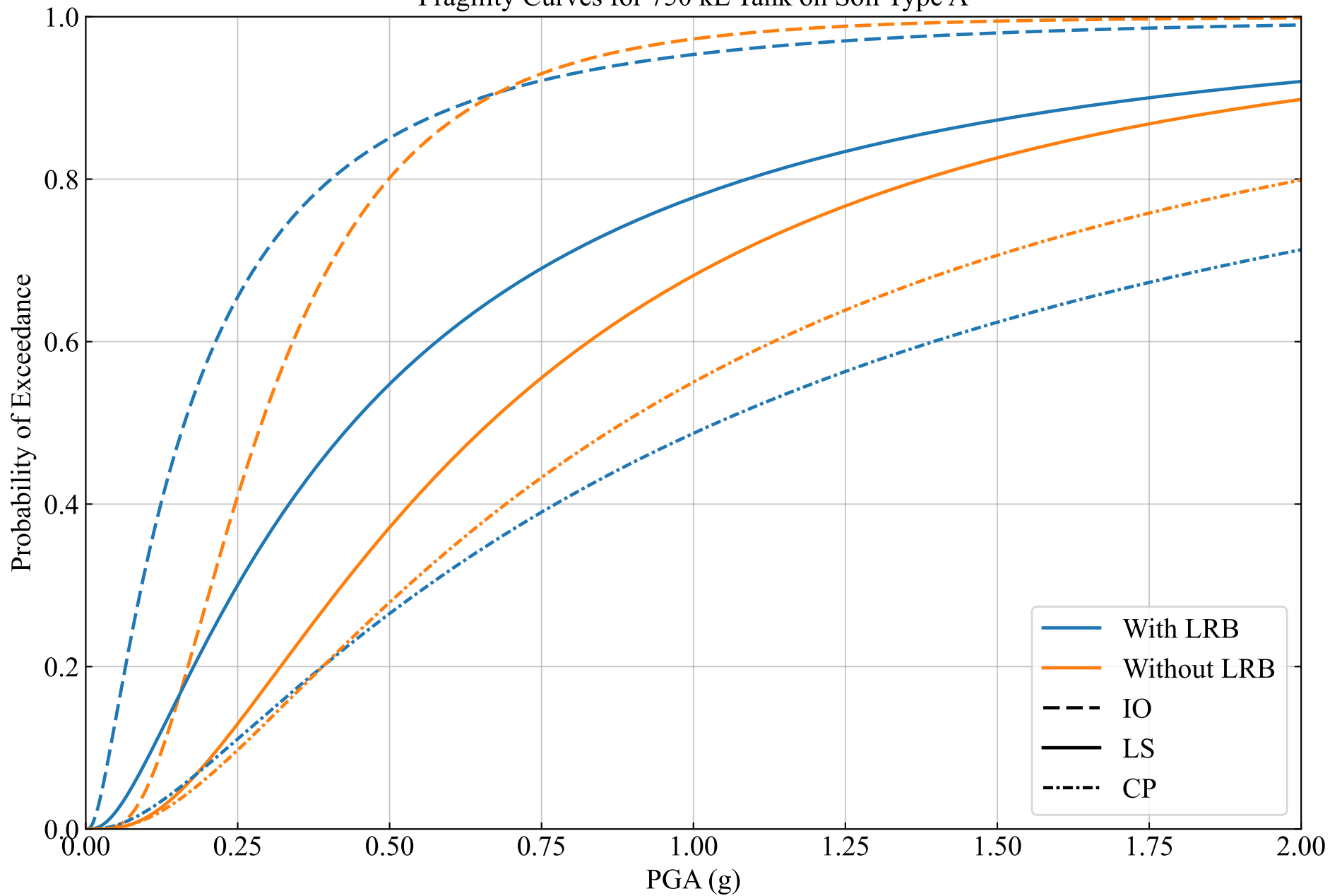
Fragility Curves for 750 kL Tank on Soil Type A
