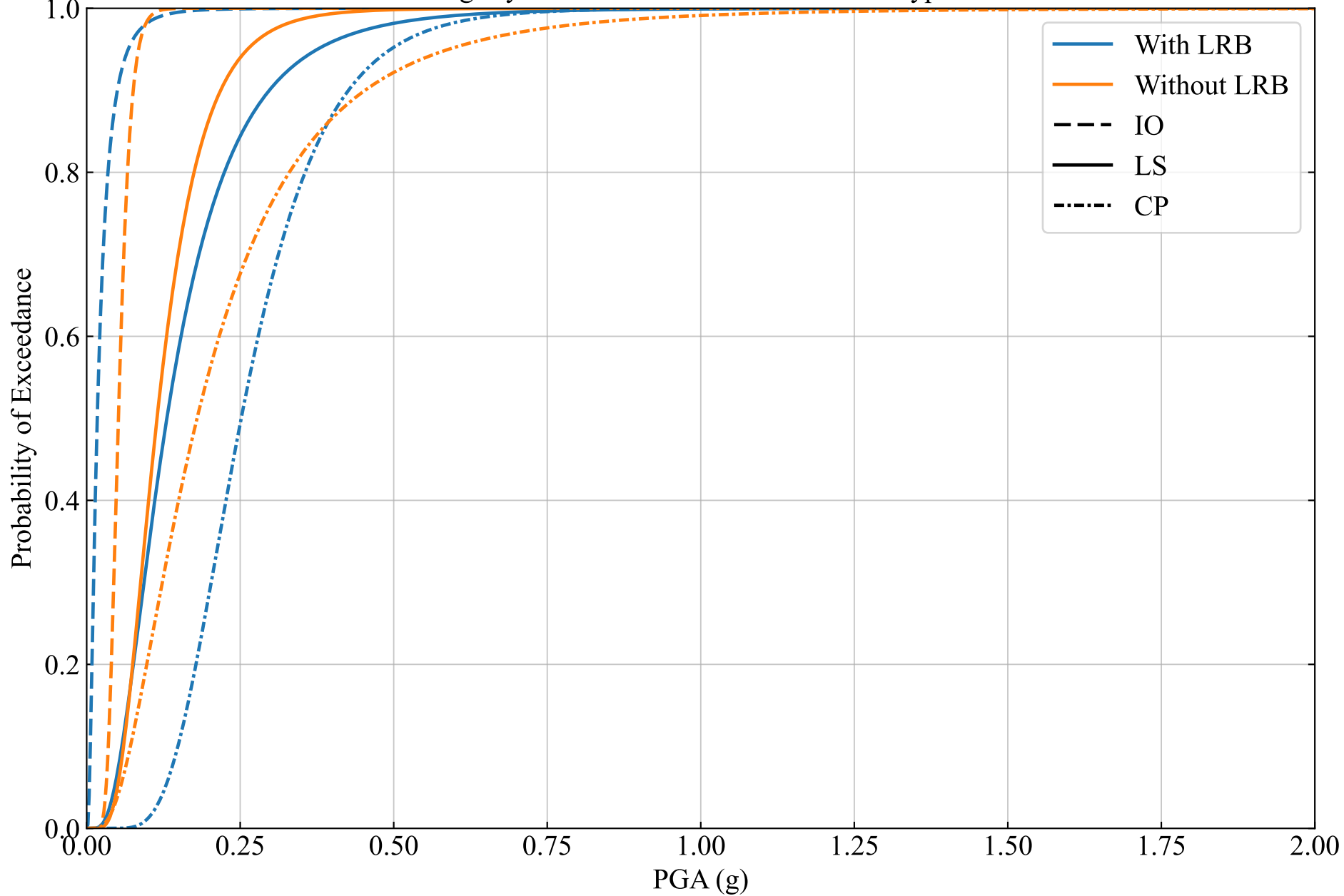
Fragility Curves for 750 kL Tank on Soil Type D
