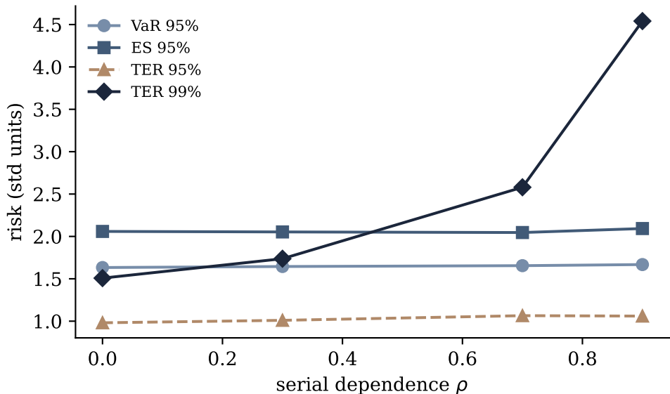
Gaussian AR(1): TER rises with clustering, VaR/ES do not
