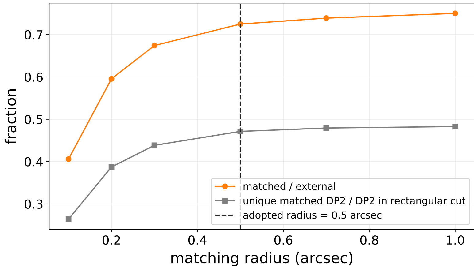
COSMOS matching-radius sweep
