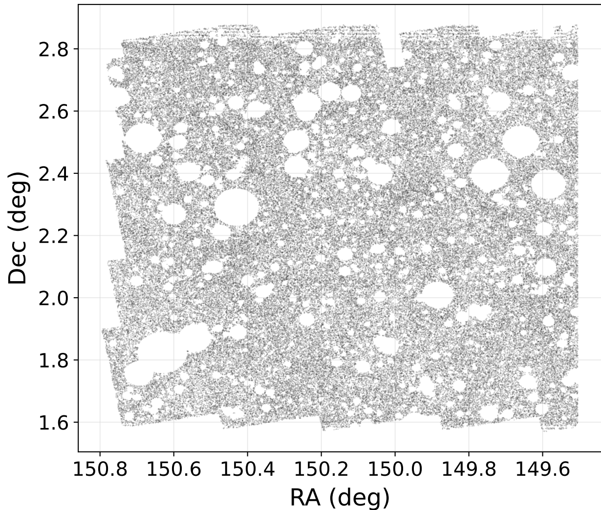
Matched COSMOS2020-DP2 paper sample
