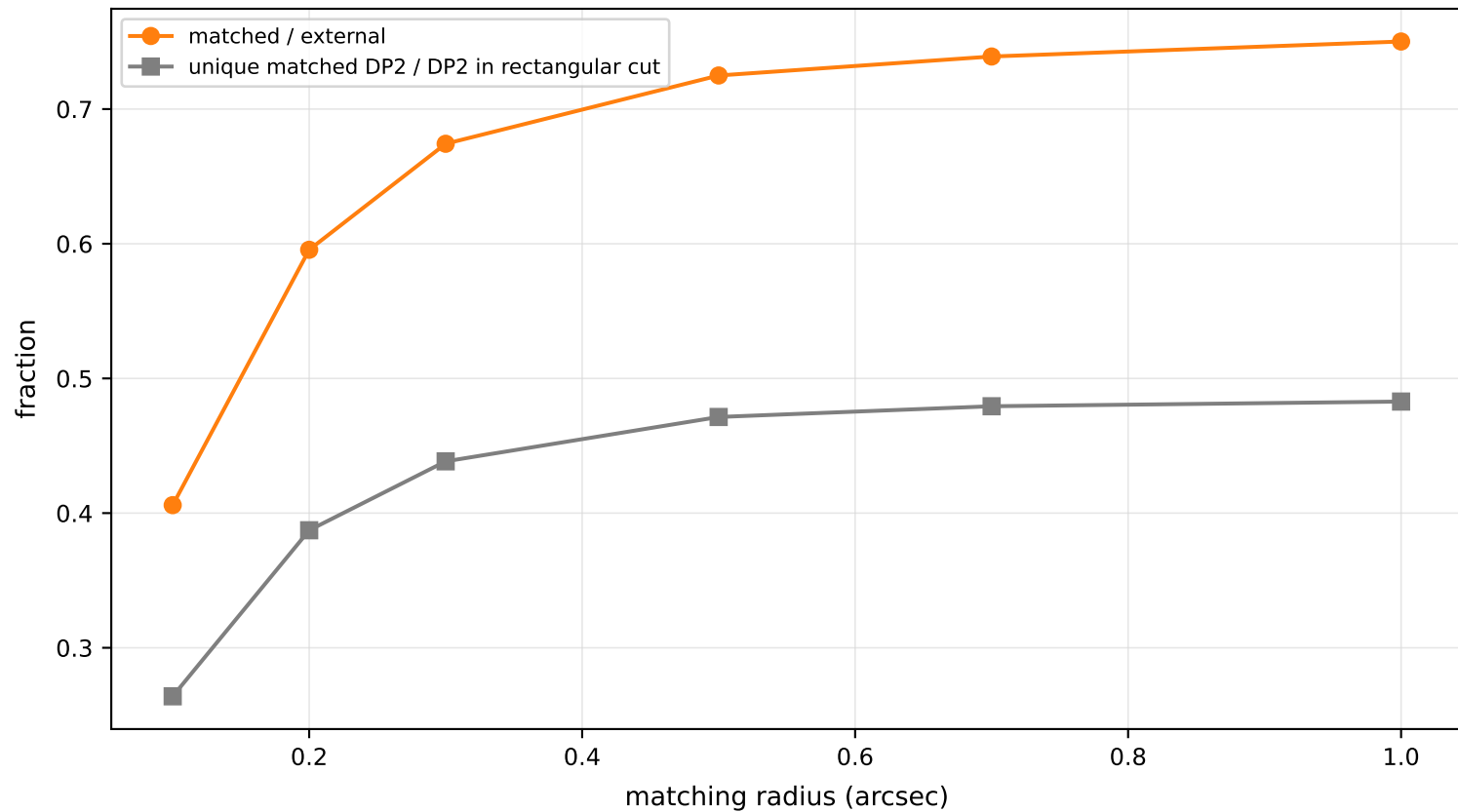
COSMOS matching-radius sweep
