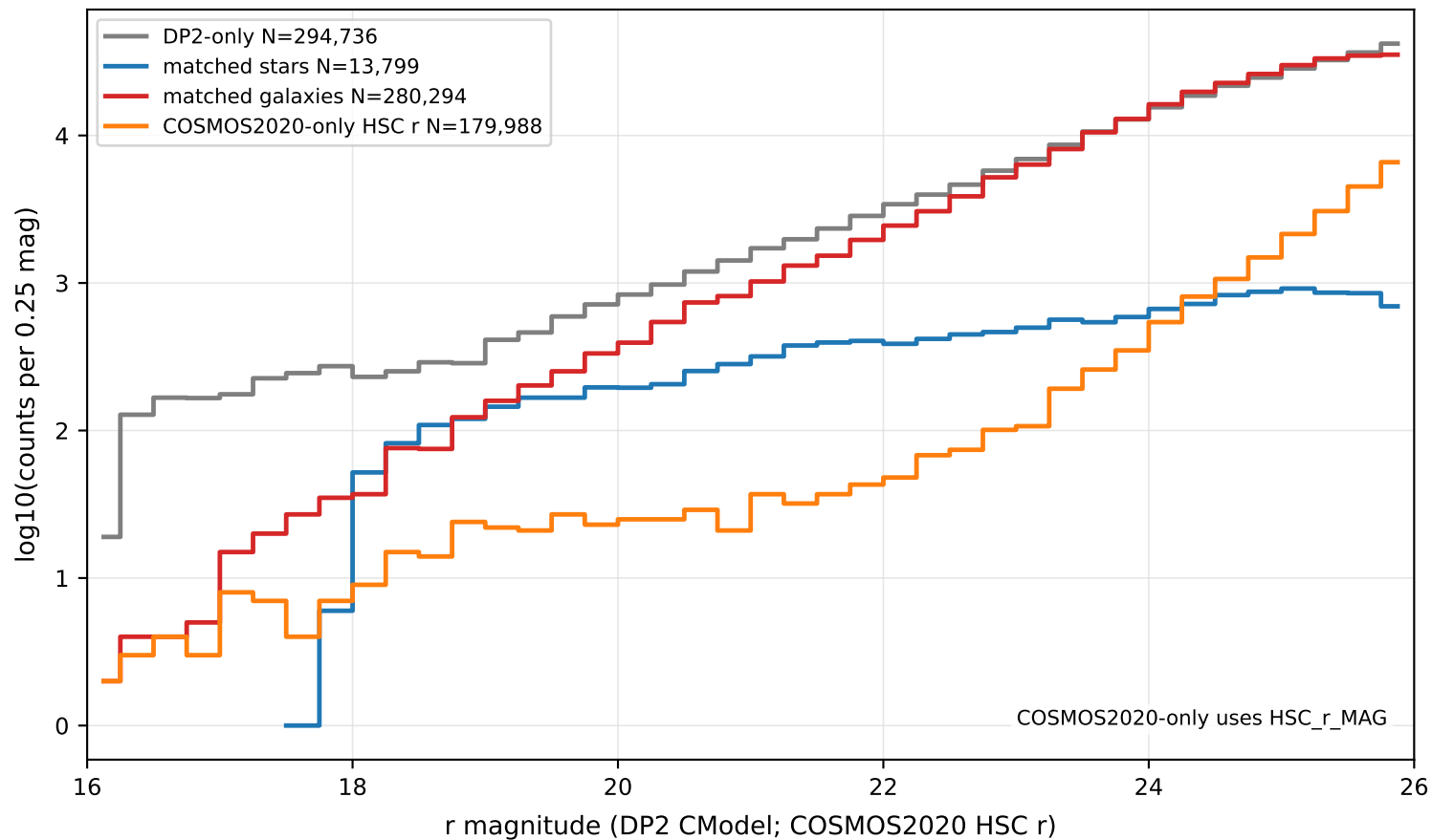
COSMOS DP2 / COSMOS2020 counts vs r magnitude, 0.25 mag bins
