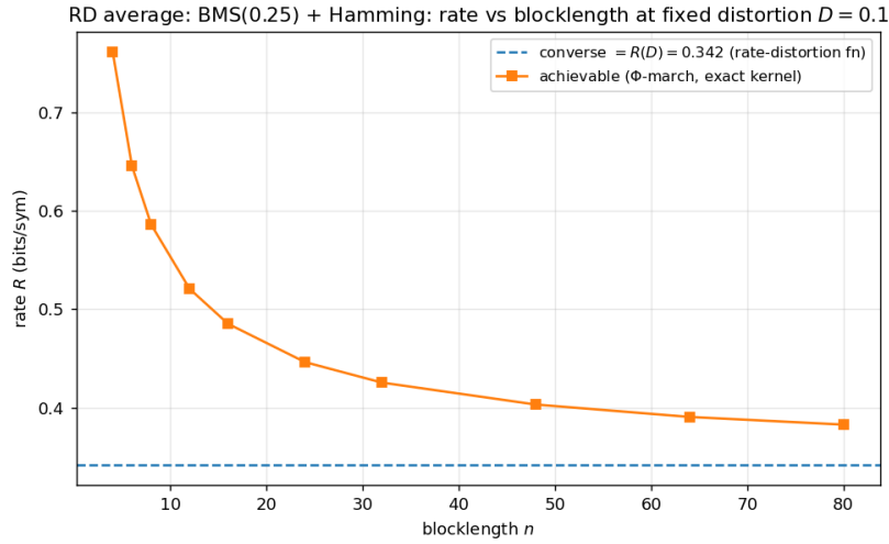
Figure 14: Rate vs. blocklength at fixed distortion D = 0.1 : the achievable rate converges from above to the converse , which for average distortion is the rate-distortion function R(D) = H(p) - H(D) = 0.342 (a valid lower bound at every n ; its dispersion term vanishes for average D ). The inversion uses the pure-NumPy march (bisection on the rate), which scales to n = 80 – past the channel’s single-cvxpy ceiling.
