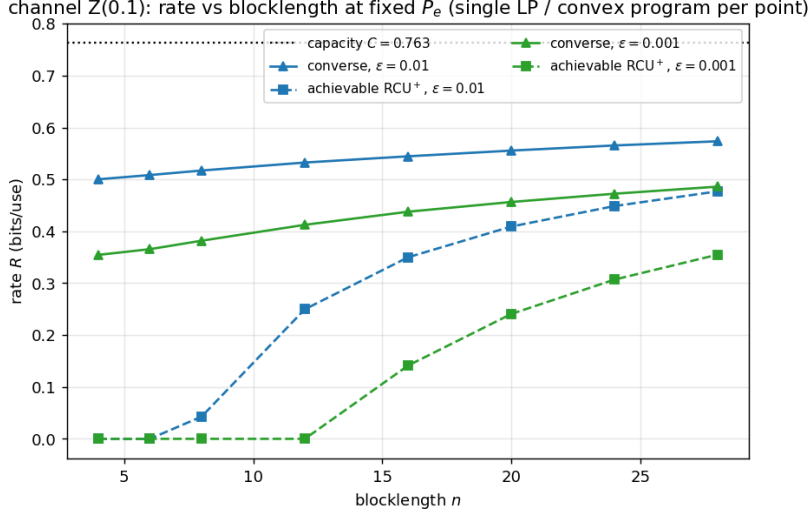
Figure 8: The complementary view: fix P_e and plot rate vs. blocklength, for two targets \epsilon = 10^{-2}, 10^{-3} (same colour = same \epsilon ; solid = converse, dashed = achievable). Both points are a single solve : the converse is one LP and the achievable \text{RCU}^+ is one convex program (the threshold w = e^{-R} enters as quad-over-linear). They bracket the \epsilon -capacity and rise toward C ; the looser \epsilon = 10^{-2} pair is higher and tighter. Capped at n = 28 by cvxpy’s compilation ceiling.
