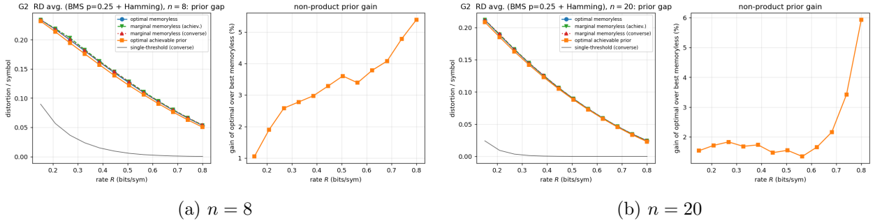
Figure 9: G2 — prior gap (exact best-of- M kernel).
