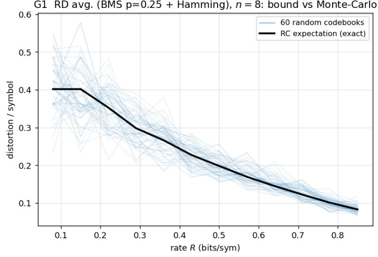
Figure 8: G1 ( n = 8 ): realized distortion vs. the random-coding expectation.
