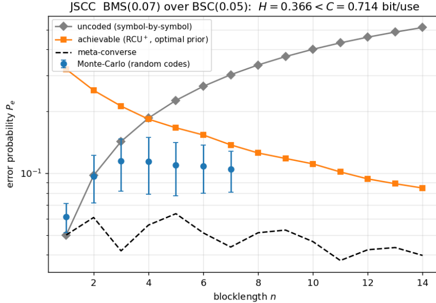
Figure 15: JSCC error probability vs. blocklength: meta-converse, achievable ( \text{RCU}^+ via the simplex march), Monte-Carlo of random codes, and the uncoded baseline.
