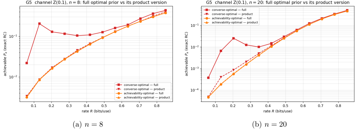
Figure 7: G5 — each optimal prior vs. its i.i.d. product (marginalized) version. The converse-optimal prior (red, full) is poor for achievability but its product collapses onto the optimum; the achievability-optimal prior is unchanged.
