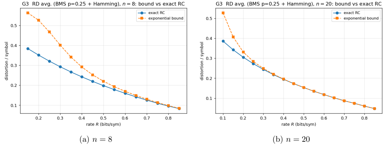
Figure 10: G3 — exact random coding vs. the exponential surrogate.
