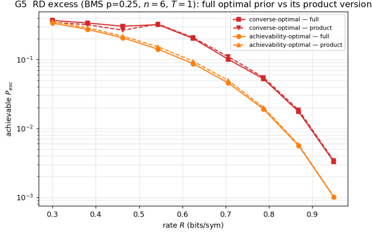
Figure 14: G5 — full vs. product prior. The converse pair sits \approx 2.8\times above the achievable pair, and—unlike channel coding—marginalizing the converse prior does not rescue it (full and product overlap).
