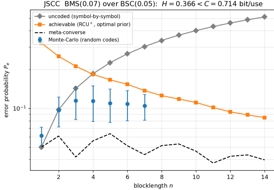
Figure 15: JSCC error probability vs. blocklength: meta-converse, achievable (RCU + via the simplex march), Monte-Carlo of random codes, and the uncoded baseline.
