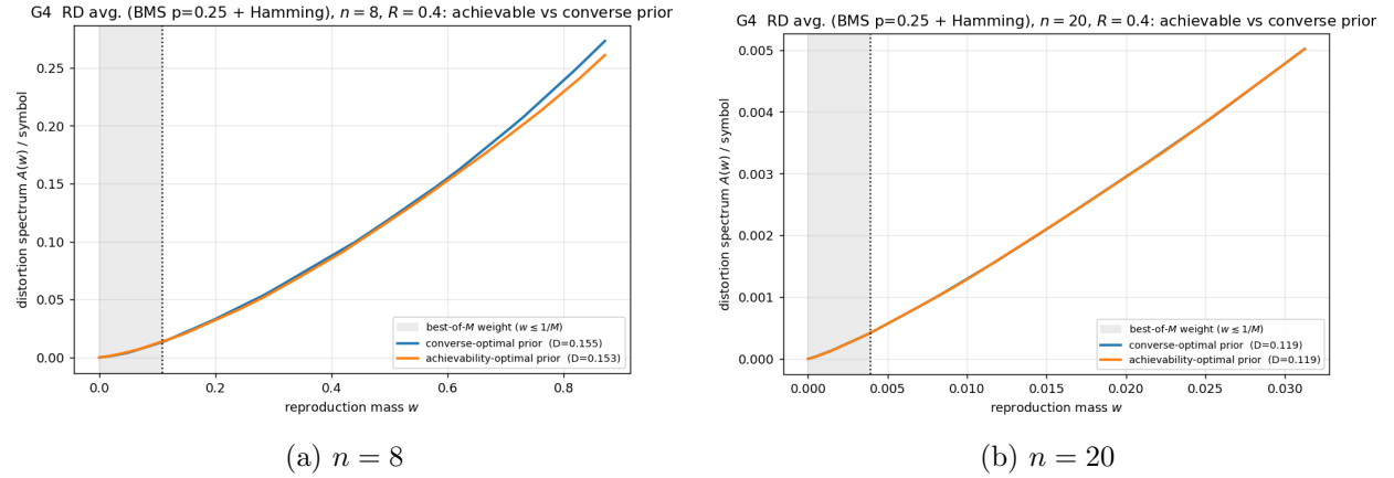
Figure 11: G4 — distortion spectra (nearly identical priors).
