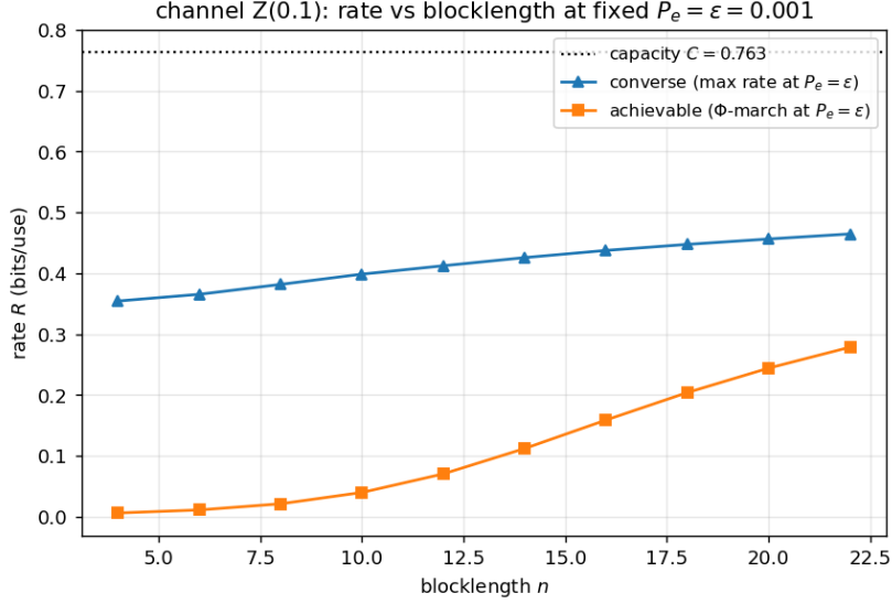
Figure 8: The complementary view: fix P_e = \epsilon = 10^{-3} and plot rate vs. blocklength. Converse (max rate with floor \leq \epsilon ) and achievable ( \Phi -march bound \leq \epsilon ) bracket the \epsilon -capacity and rise toward C . Each point is a bisection on R (the bound is monotone in rate).
