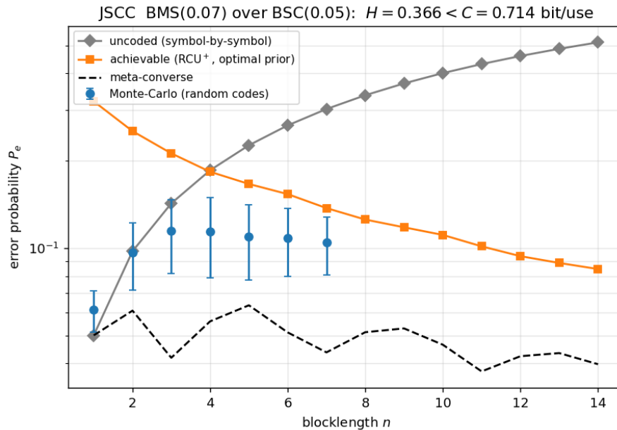
Figure 16: JSCC error probability vs. blocklength: meta-converse, achievable ( \text{RCU}^+ via the simplex march), Monte-Carlo of random codes, and the uncoded baseline.
