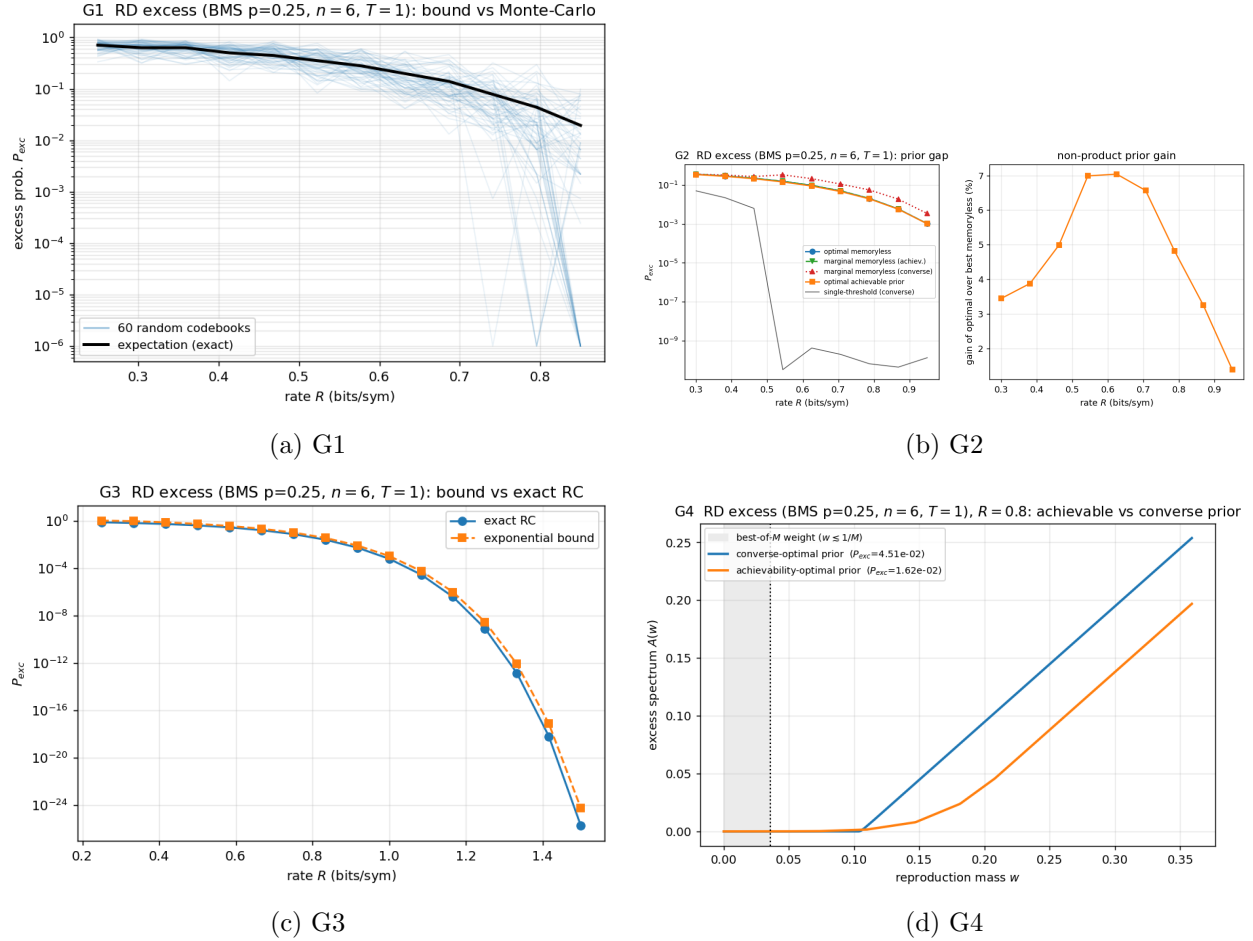
Figure 14: Excess distortion: bound vs. MC (G1), prior gap (G2), exact vs. bound (G3), and the excess spectra (G4); the converse-marginal prior is the worst here.
