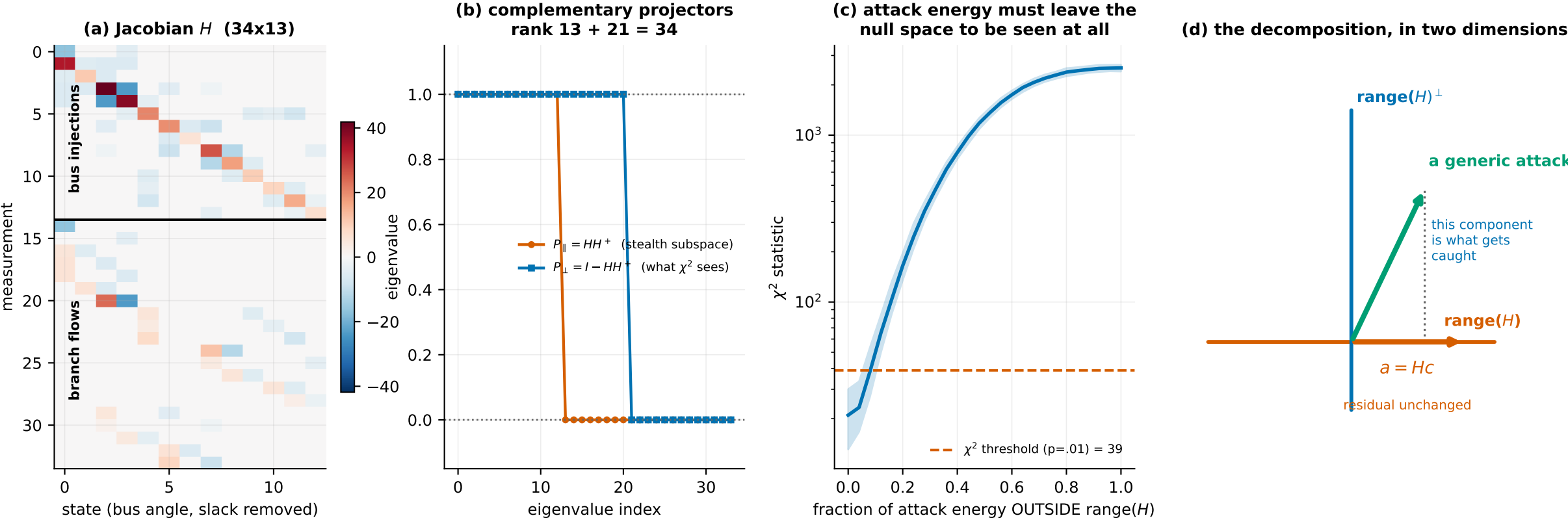
Figure 2 -- Why stealth is a property of linear algebra, not of attacker cleverness. Any injection lying in \text{range}(H) leaves the state-estimation residual exactly unchanged.
