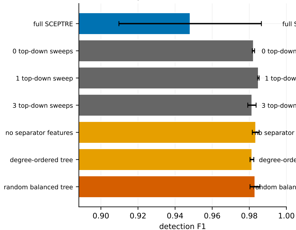
(a) component ablation -- detection
