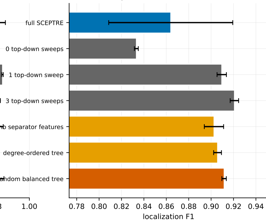
(b) component ablation -- localization
