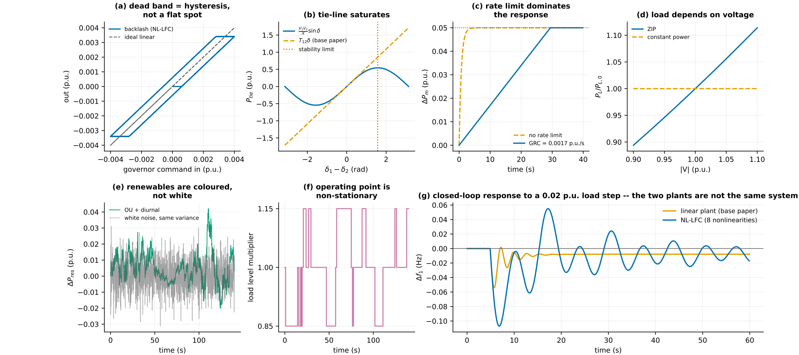
Figure 5 -- The eight NL-LFC mechanisms, isolated. Panels (a)-(f) show each in its own right; panel (g) shows what they do together, which is what a detector actually has to cope with.
