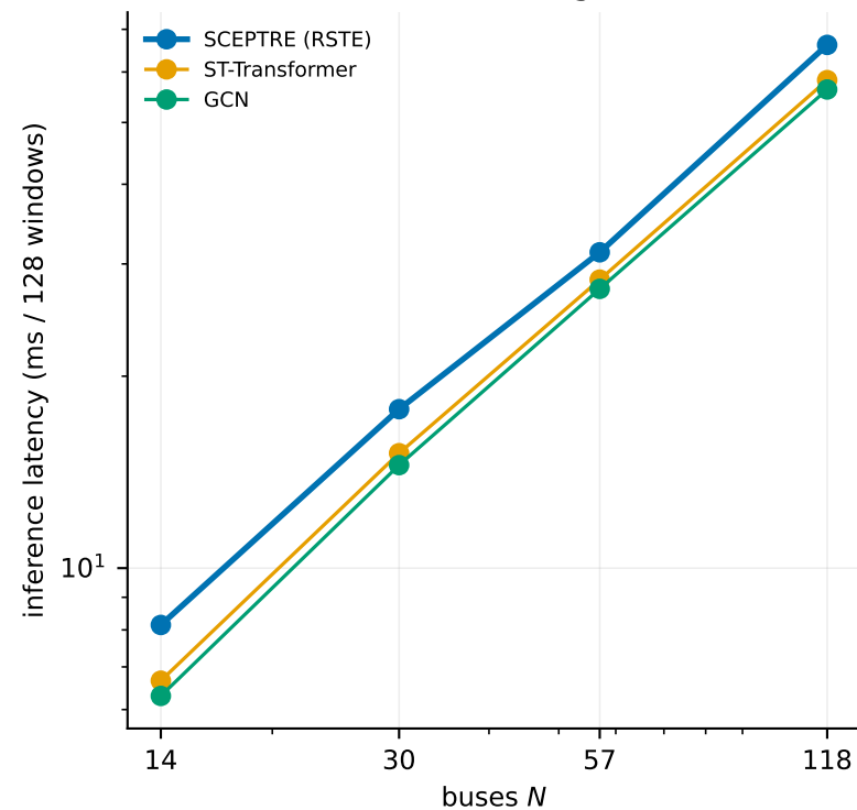
(c) measured cost scaling on RTX 5060
