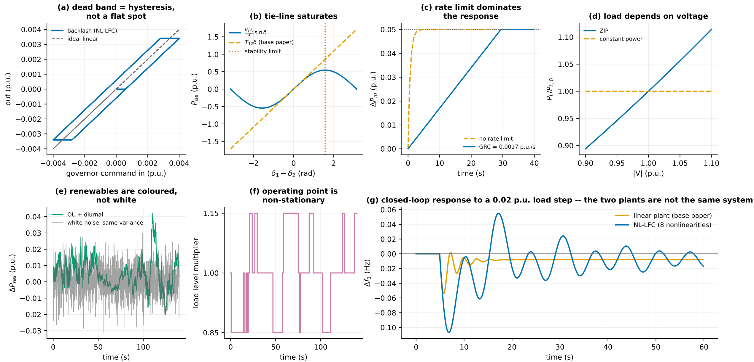
Figure 5 -- The eight NL-LFC mechanisms, isolated. Panels (a)-(f) show each in its own right; panel (g) shows what they do together, which is what a detector actually has to cope with.
