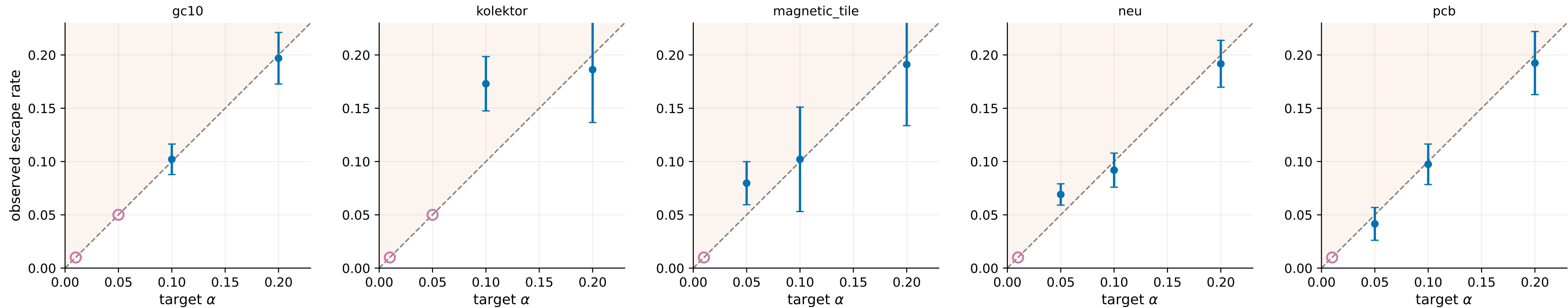
Conformal risk control holds across all five domains (60 repeated splits)
