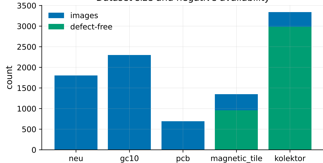
Dataset size and negative availability
