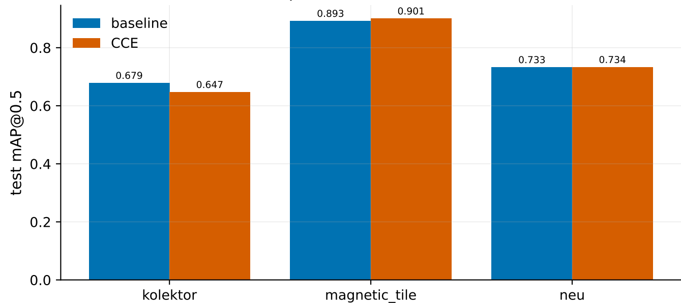
CCE ablation (paired, same model/dataset/seed)
