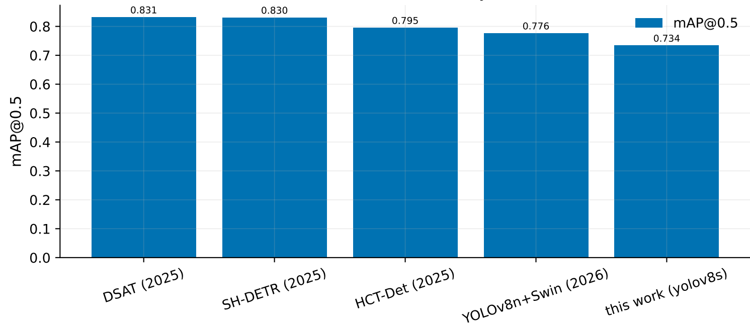
NEU-DET — detection accuracy in context
