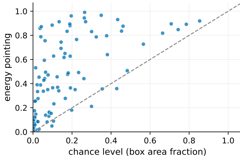
above the diagonal = better than chance
