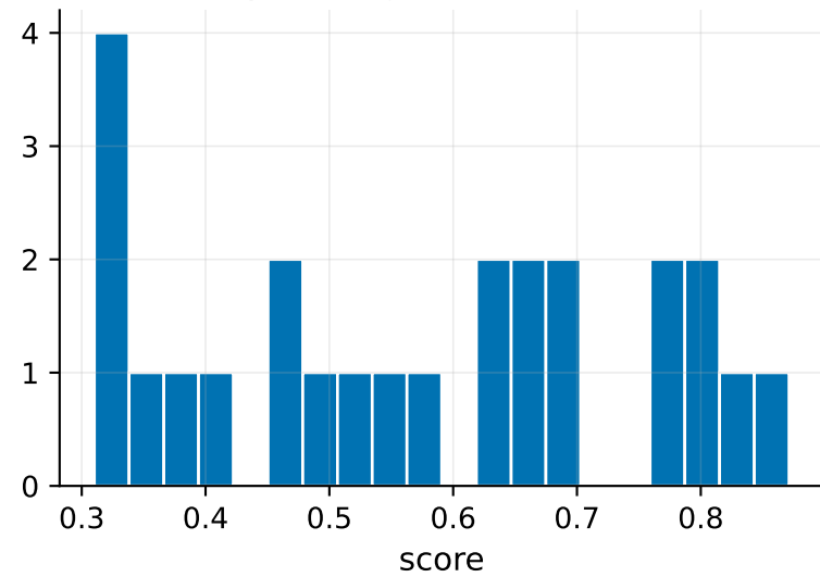
per-image faithfulness
