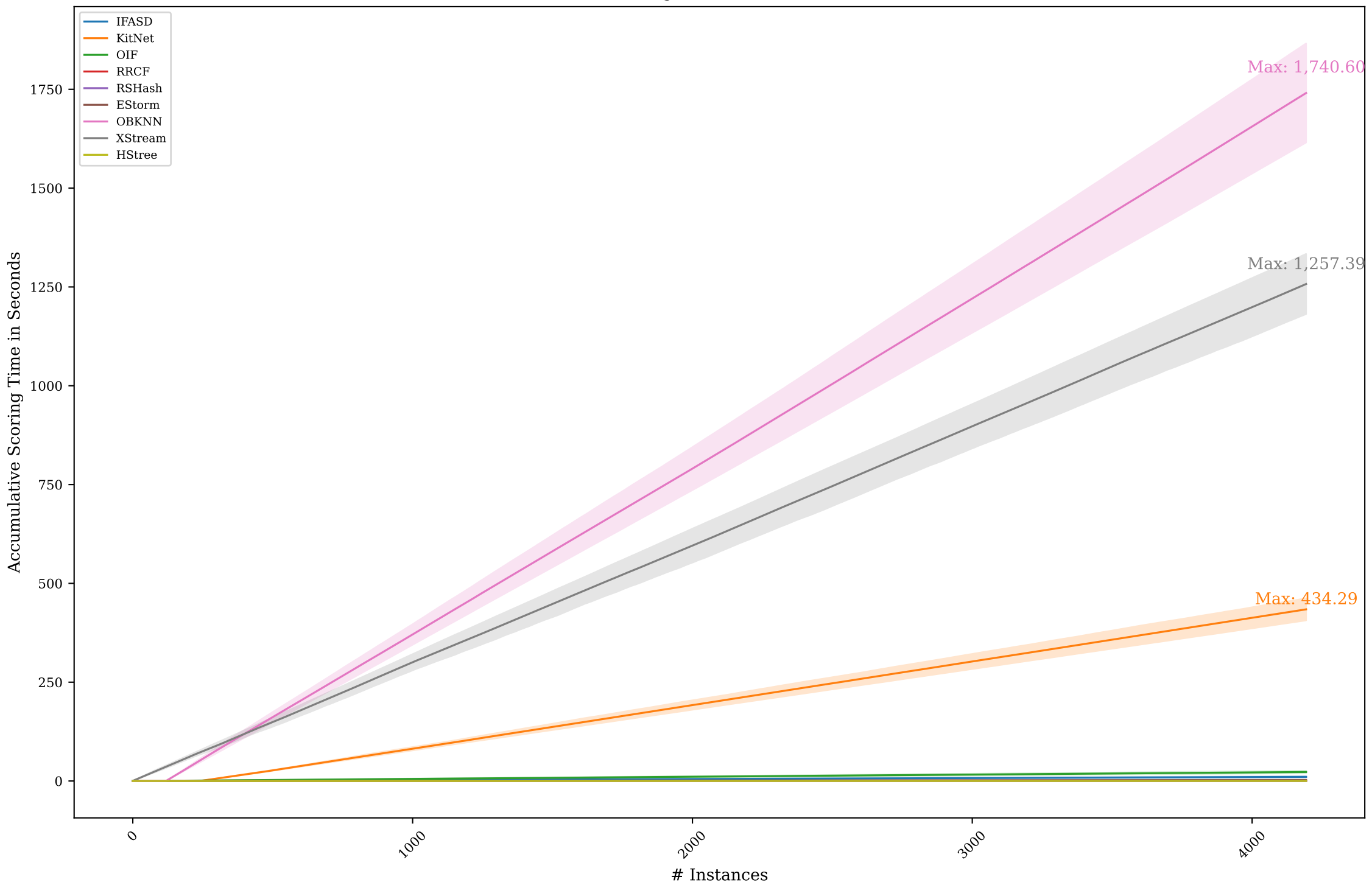
Scoring Time: Scenario A1
