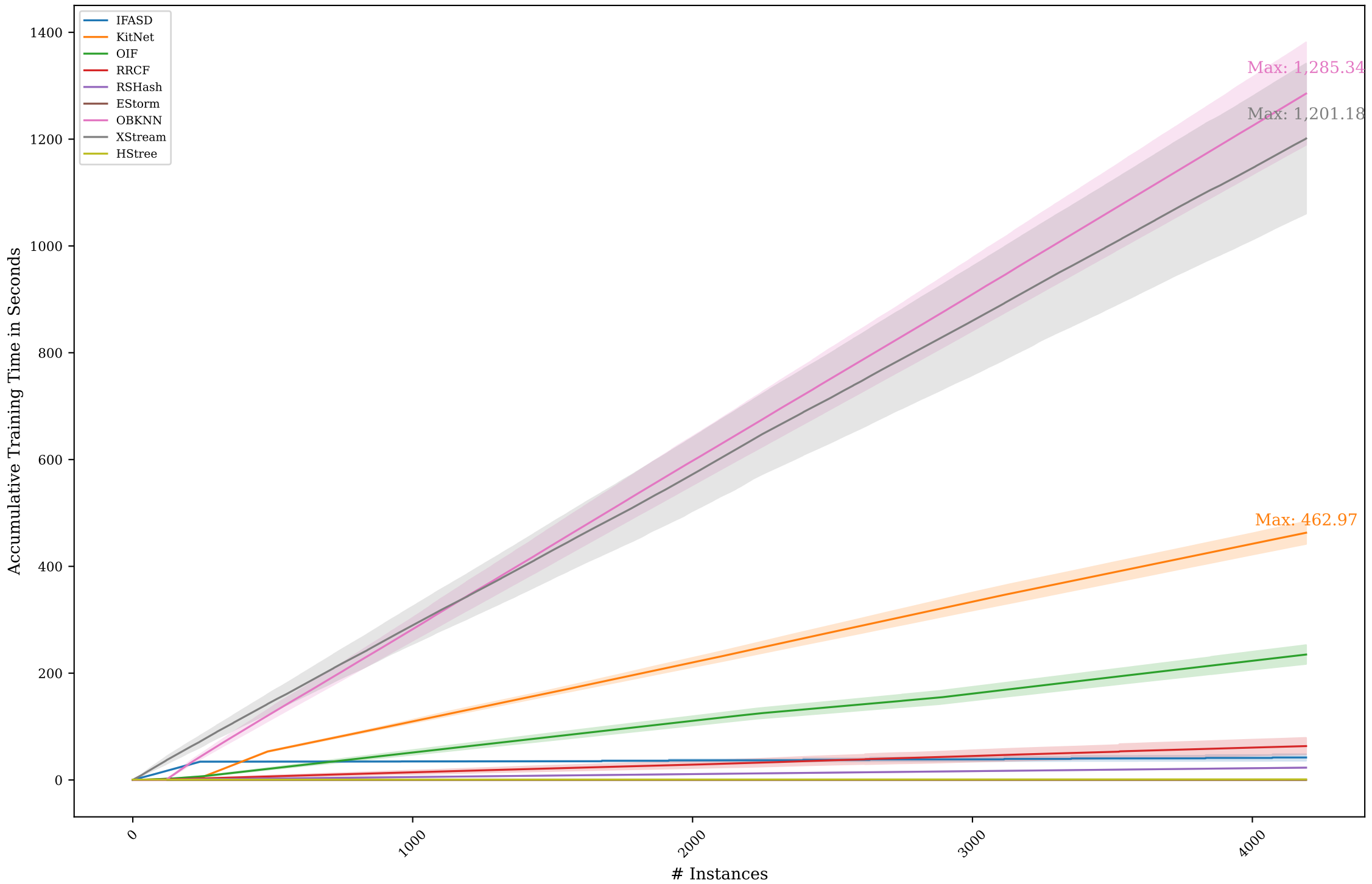
Training Time: Scenario A3
