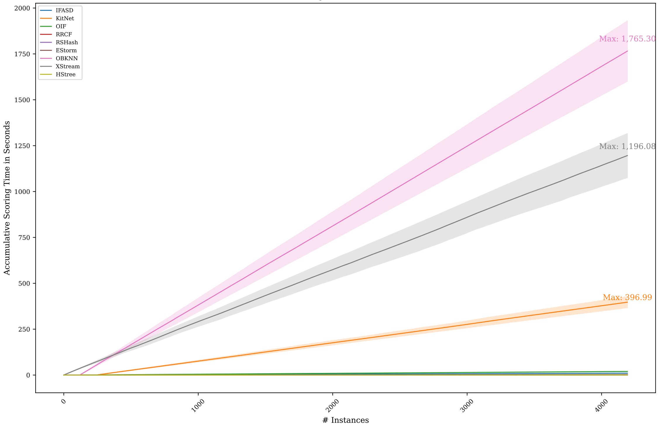
Scoring Time: Scenario A4
