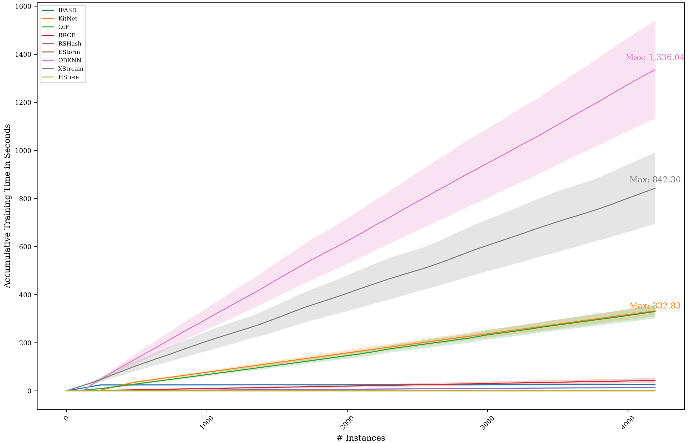
Training Time: Scenario A9
