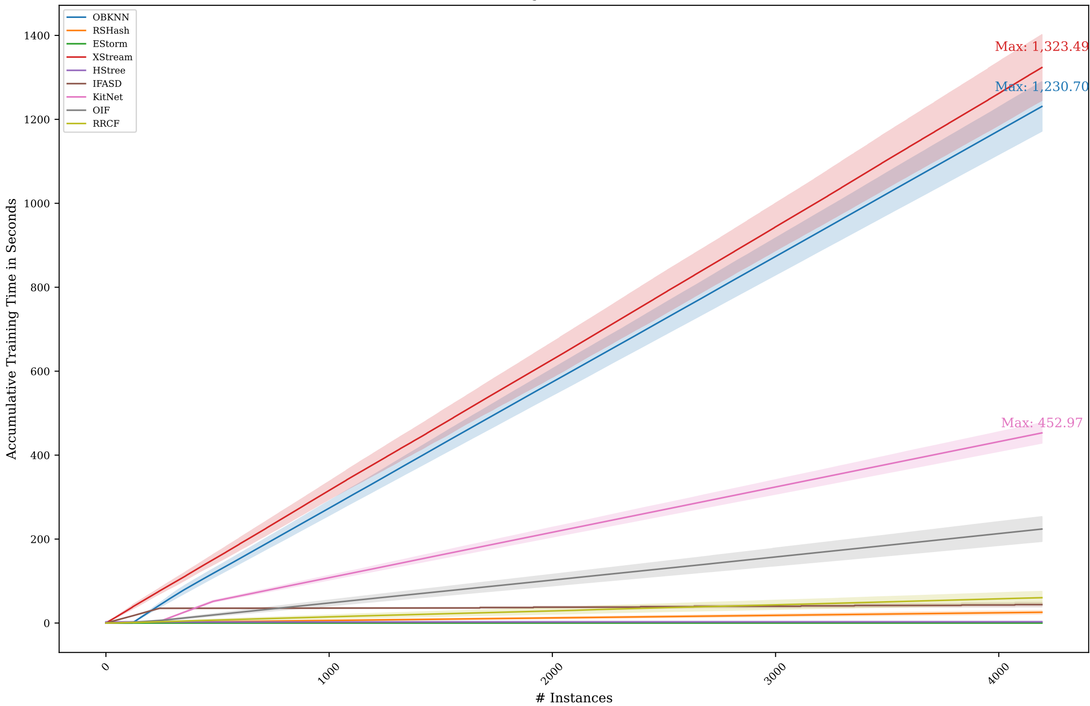
Training Time: Scenario A1
