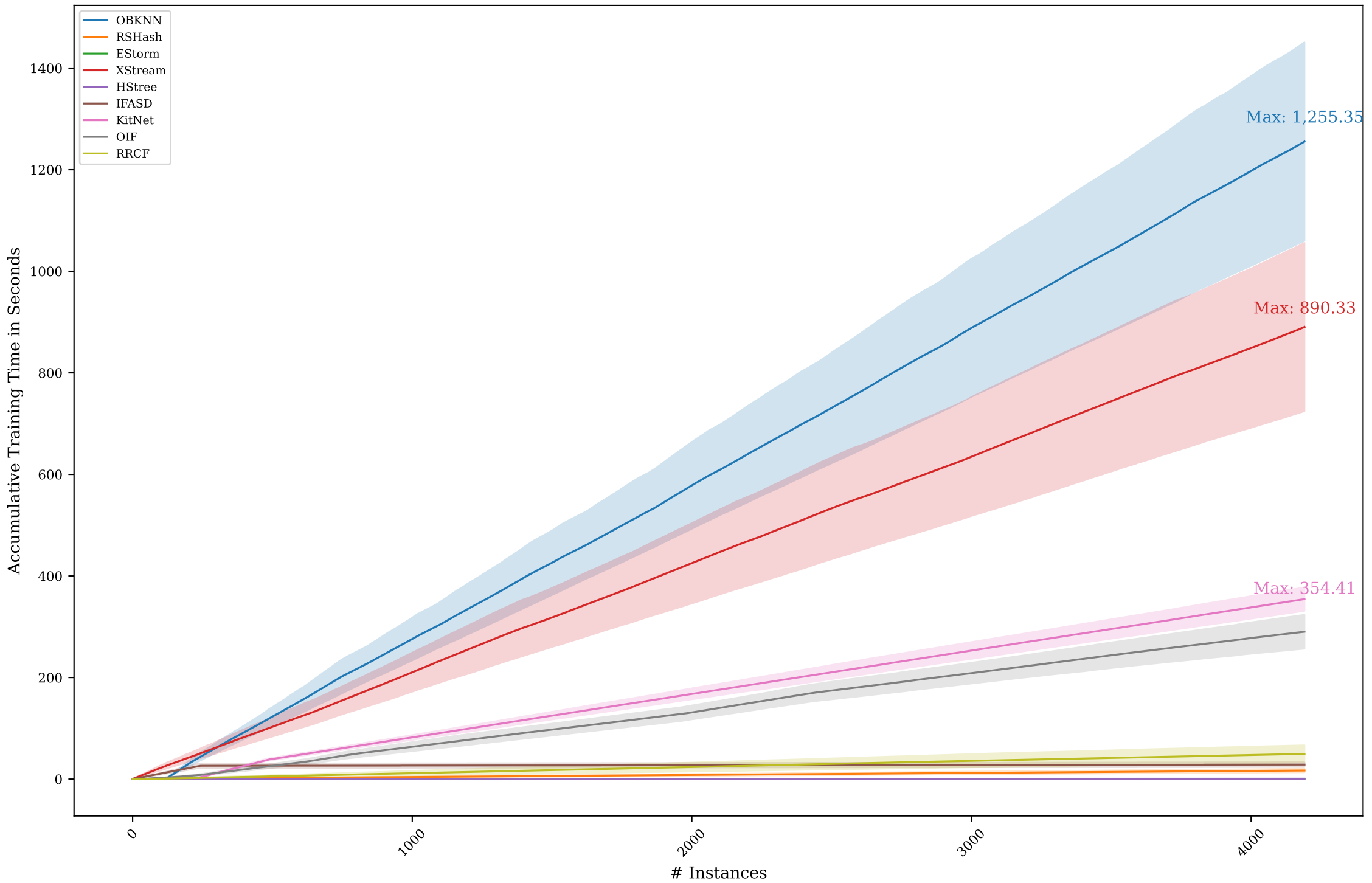
Training Time: Scenario A7
