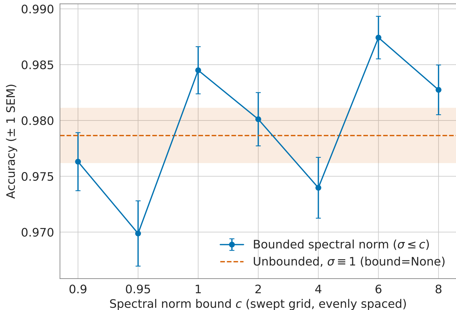
SNGP on Acevedo test (n = 3,419)
