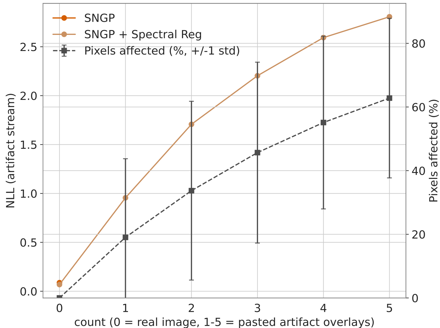
Config axis: NLL and pixel coverage vs. overlay count
