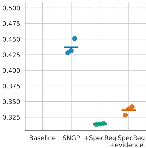
GP-variance AUROC vs CIFAR-10 ↑
