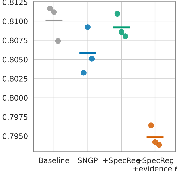
GP-variance AUROC vs SVHN ↑
