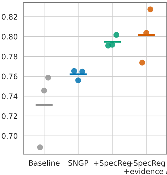
MSP AUROC vs SVHN ↑
