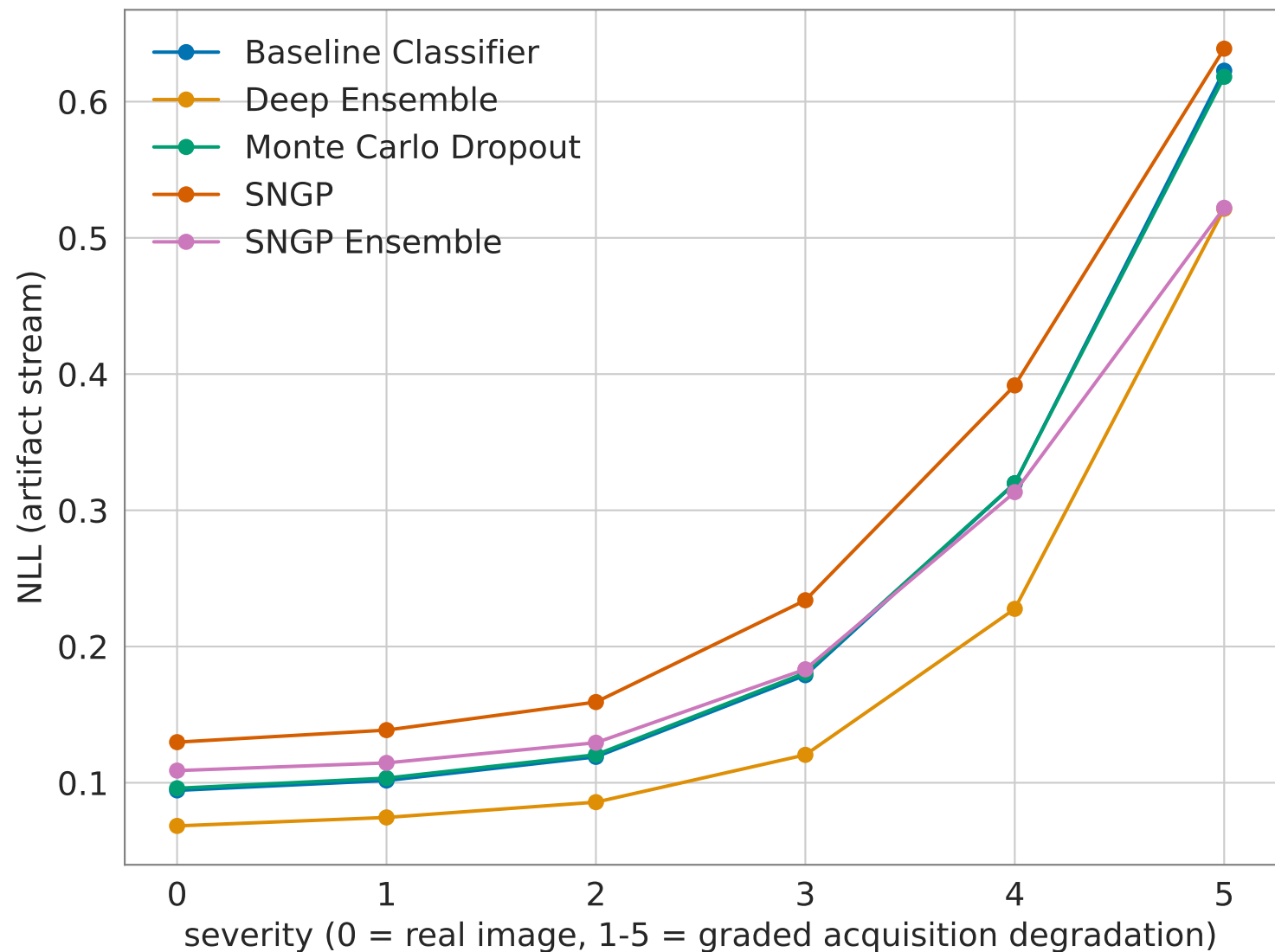
Procedural axis: NLL vs. severity
