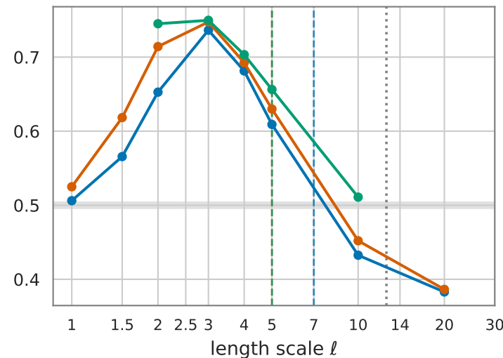
Variance AUROC vs CIFAR-10 \uparrow
