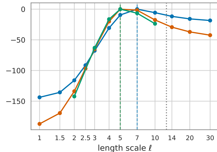
Type-II log evidence / N, train ( \Delta from max) \uparrow
