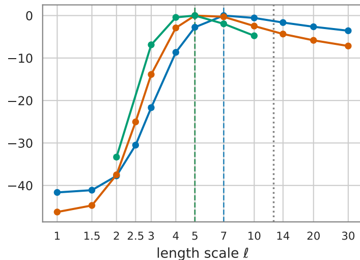
Type-II log evidence / N, val ( \Delta from max) \uparrow
