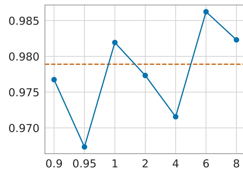
Recall (macro)
