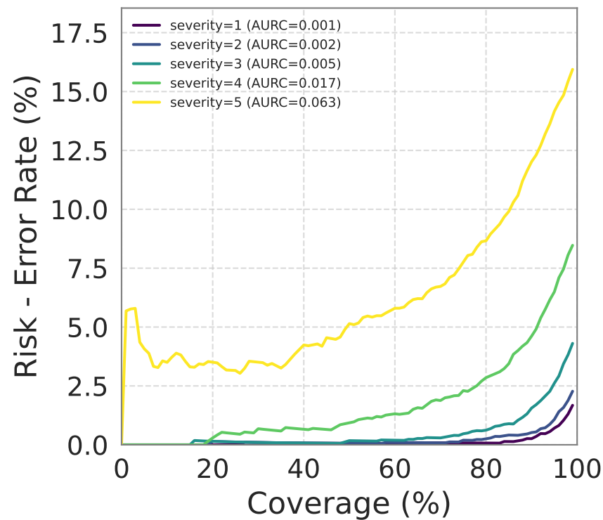
Baseline Classifier
