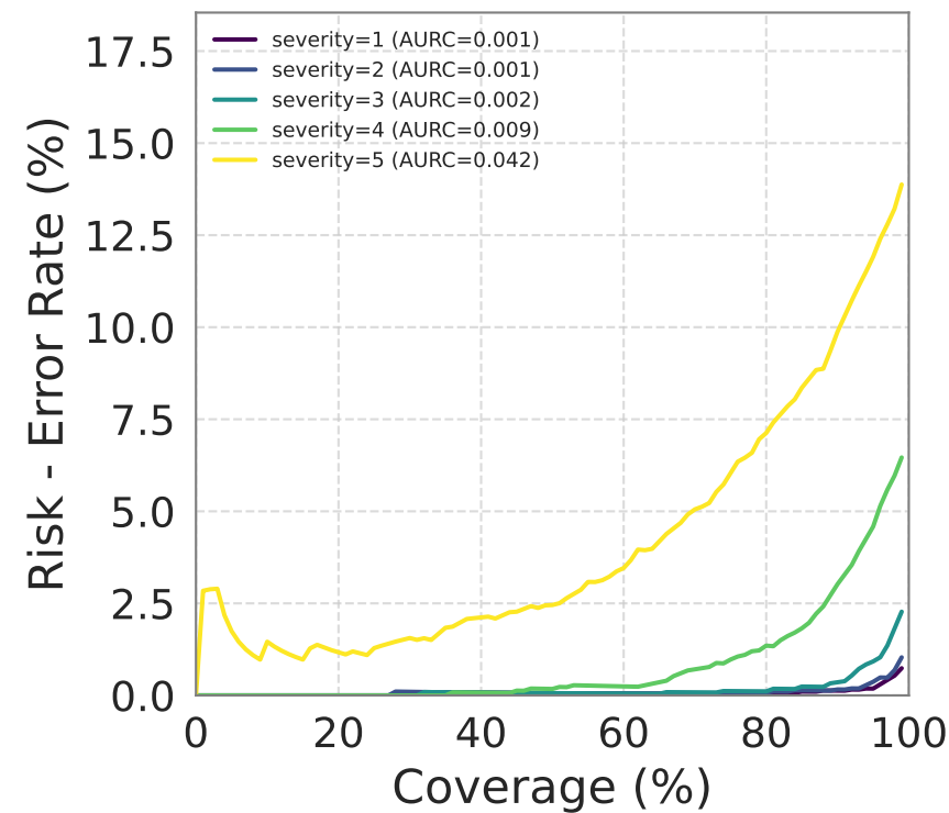
Deep Ensemble
