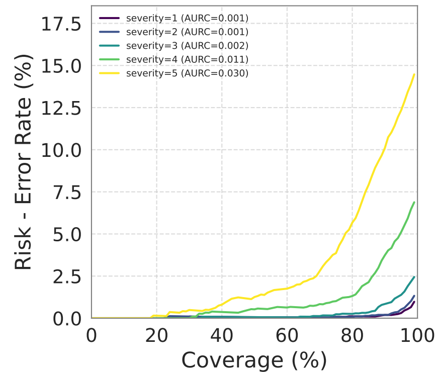
SNGP Ensemble
