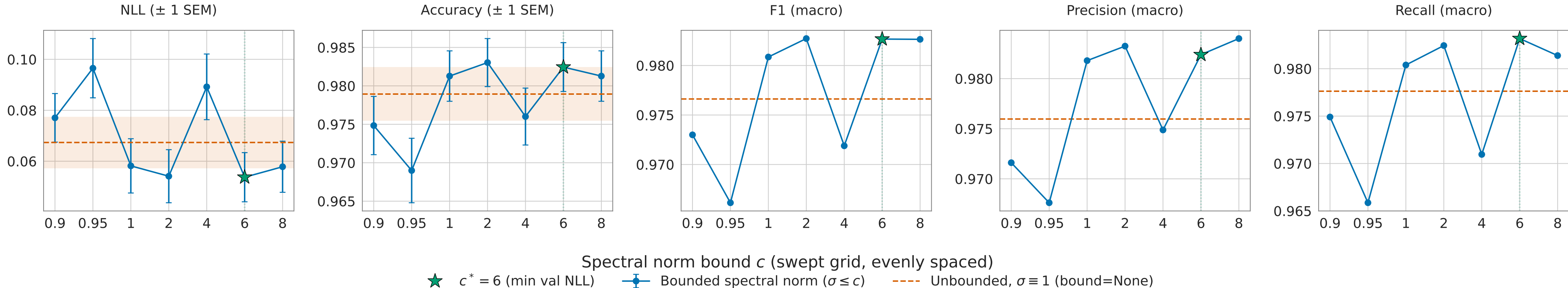
SNGP on Acevedo val (n = 1,709), c^* = 6
