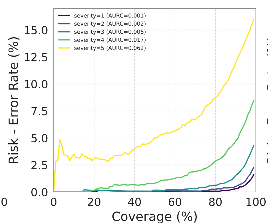
Monte Carlo Dropout
