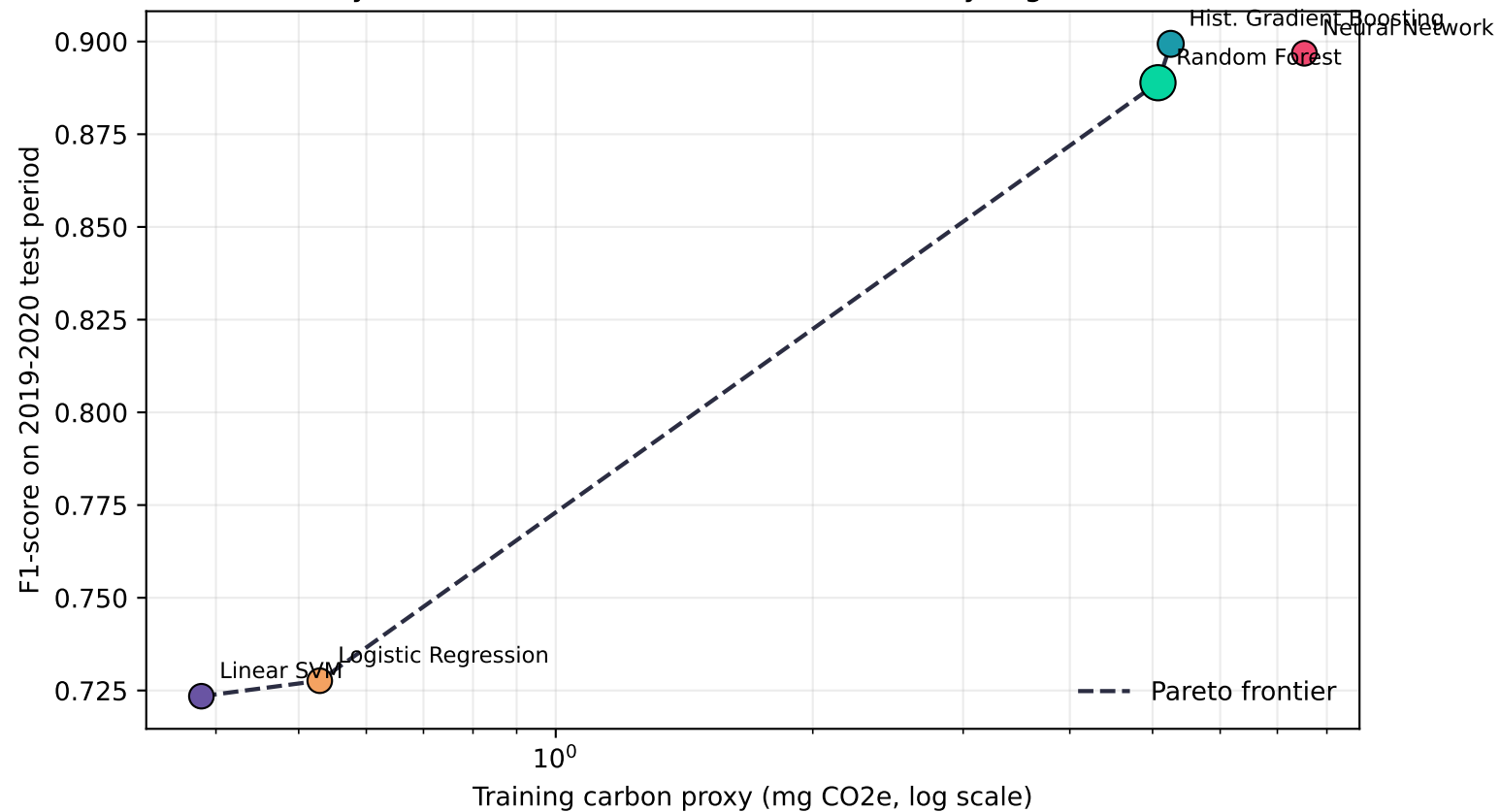
RQ1: Accuracy-Carbon Trade-off for German Next-Day High-Load Classification
