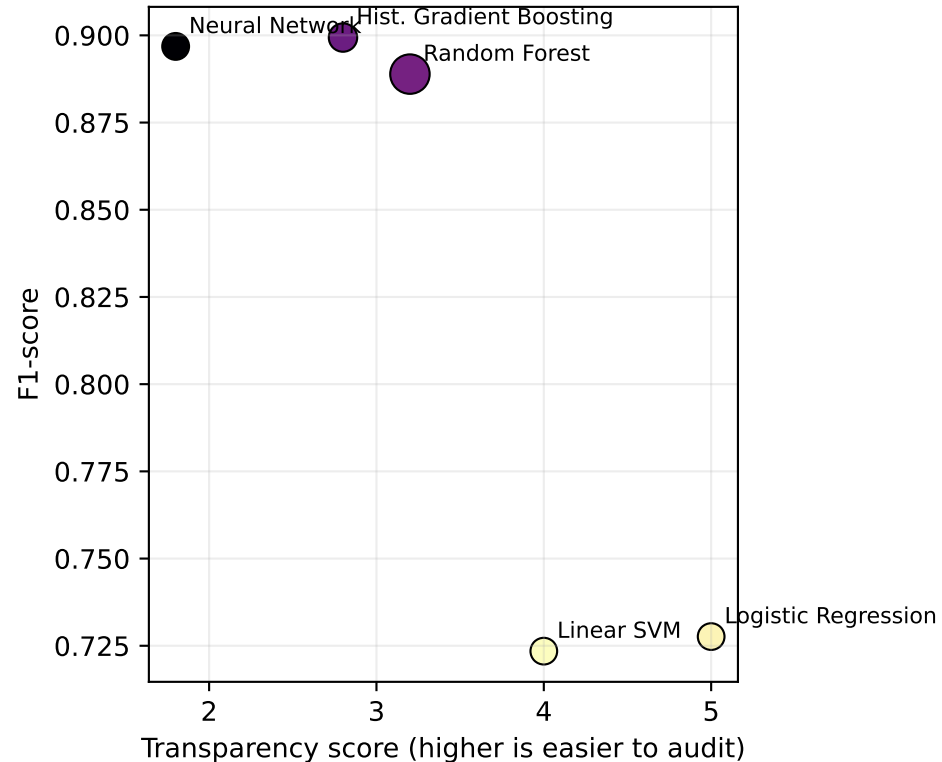
Accuracy versus auditability
