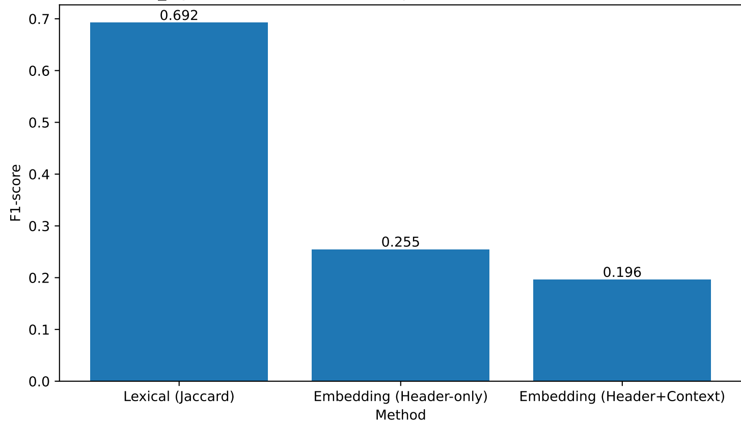
RQ1_Fig1 — Overall F1-score Comparison (Ground Truth Evaluation)
