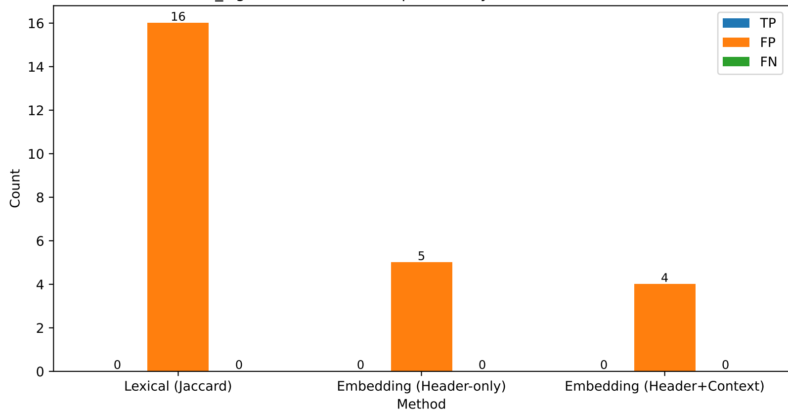
RQ1_Fig3 — Confusion Components by Method (TP / FP / FN)
