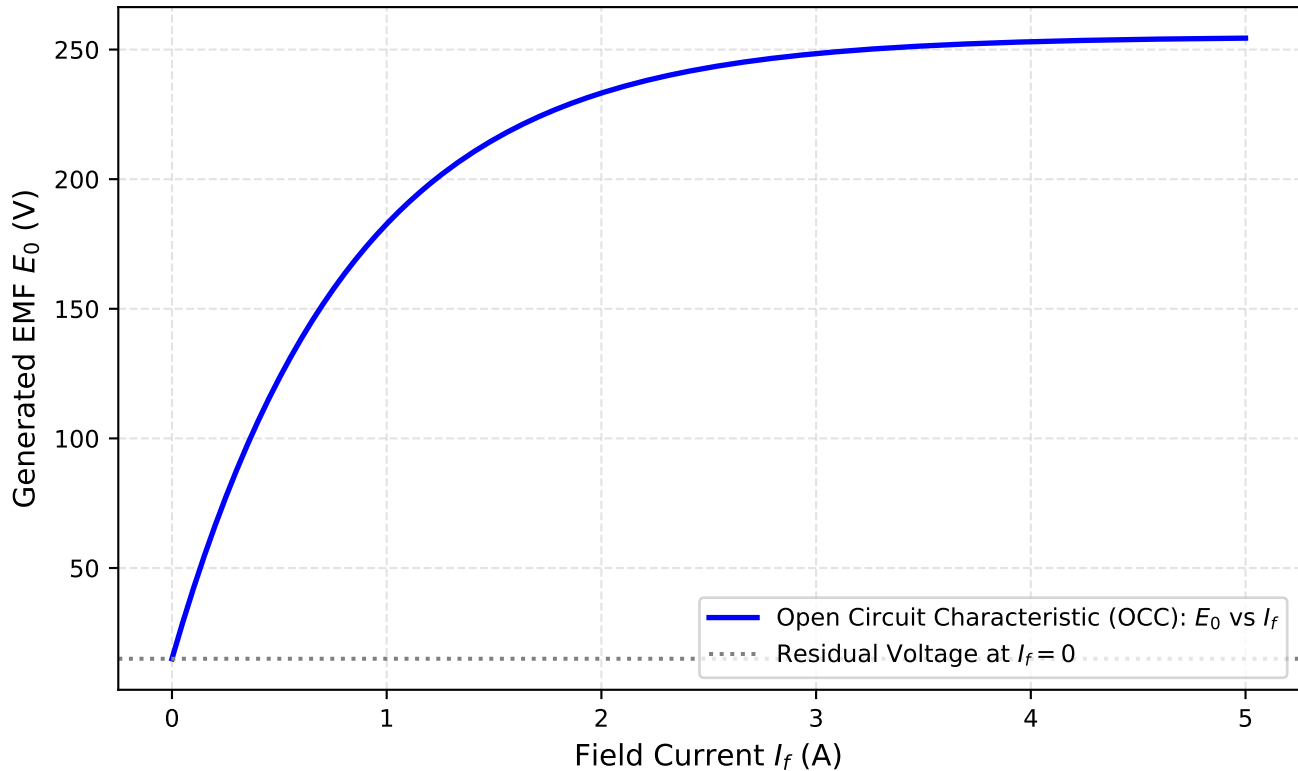
DC Generator Open-Circuit Magnetization Curve (OCC)
