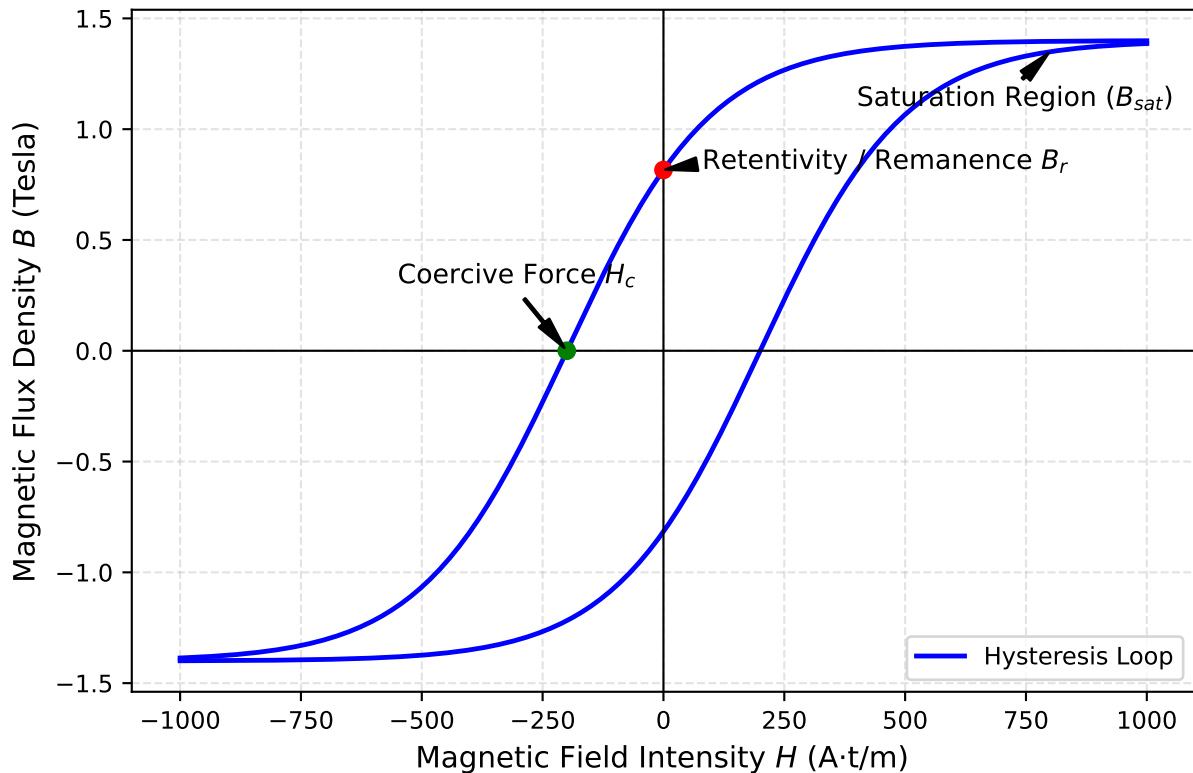
Ferromagnetic Material B - H Hysteresis Loop
