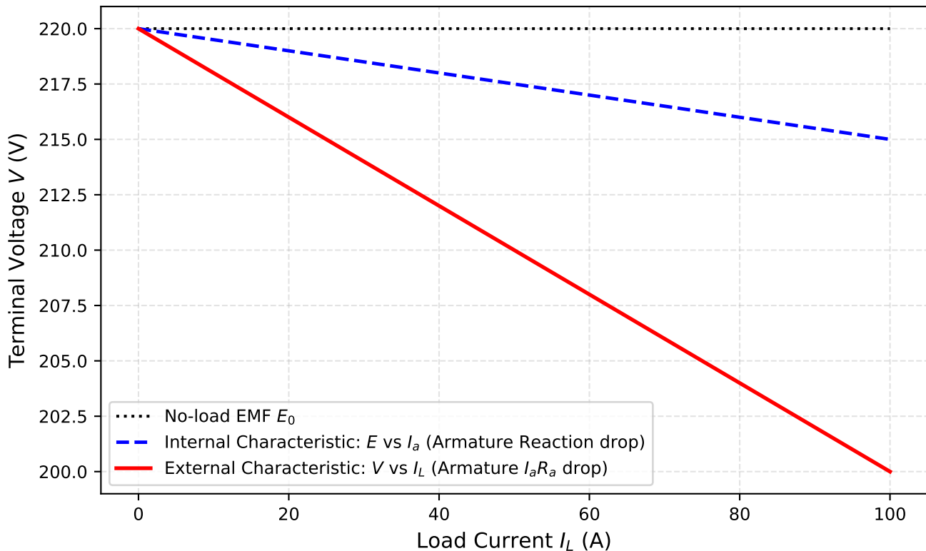
DC Shunt Generator Internal and External Characteristics
