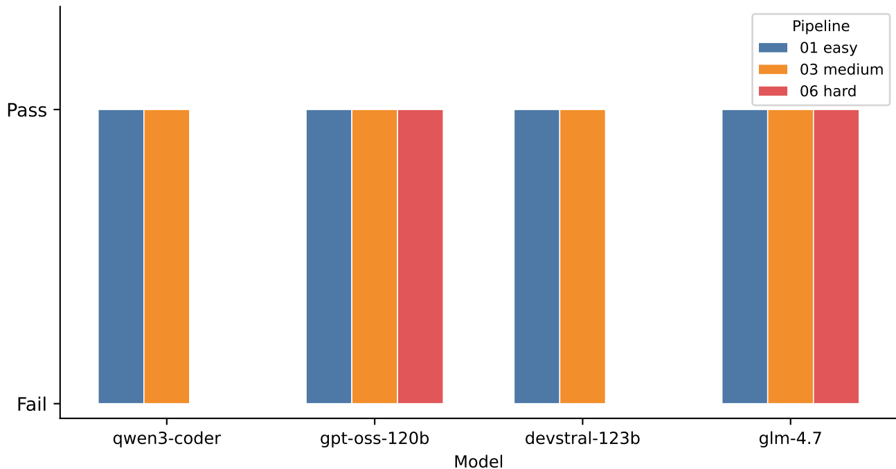
Cross-model comparison — dynamic pass per pipeline
