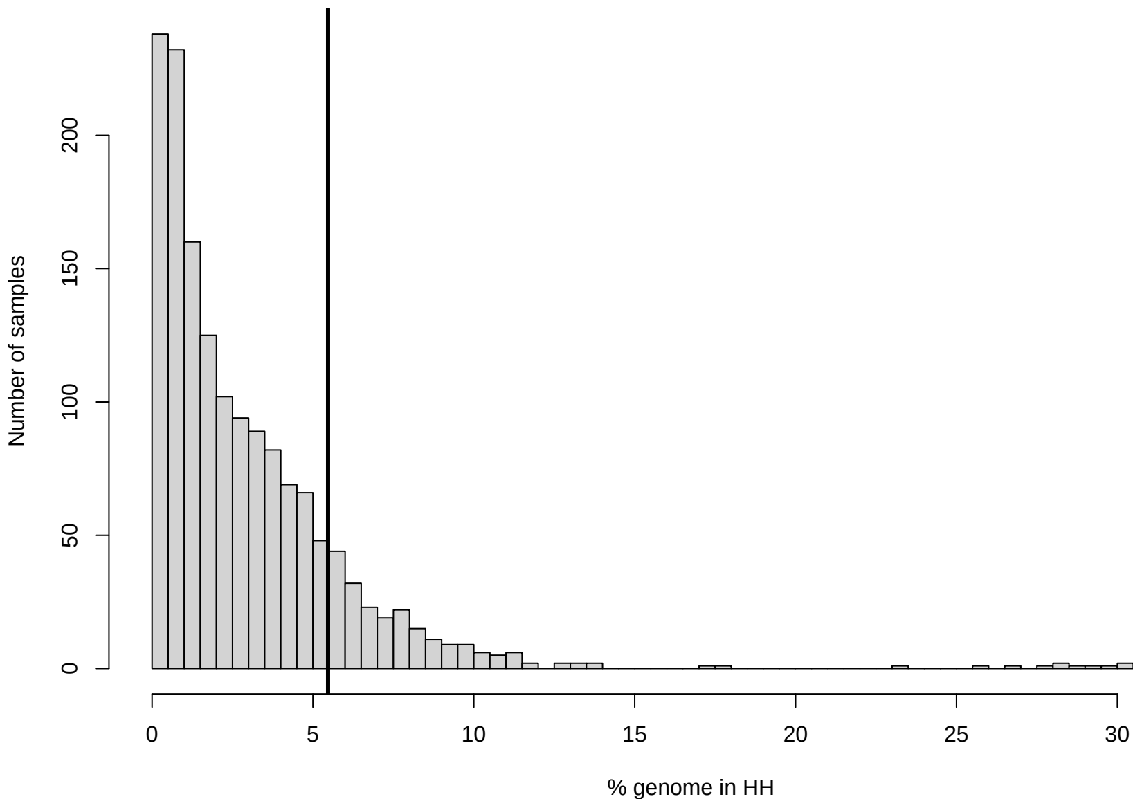
Observed donor % (HH only) vs expected BC2S3
