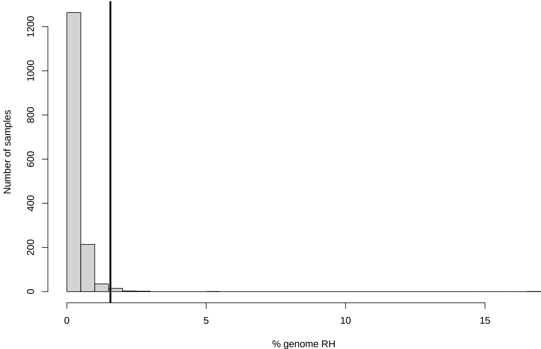
Observed RH % vs expected BC2S3
