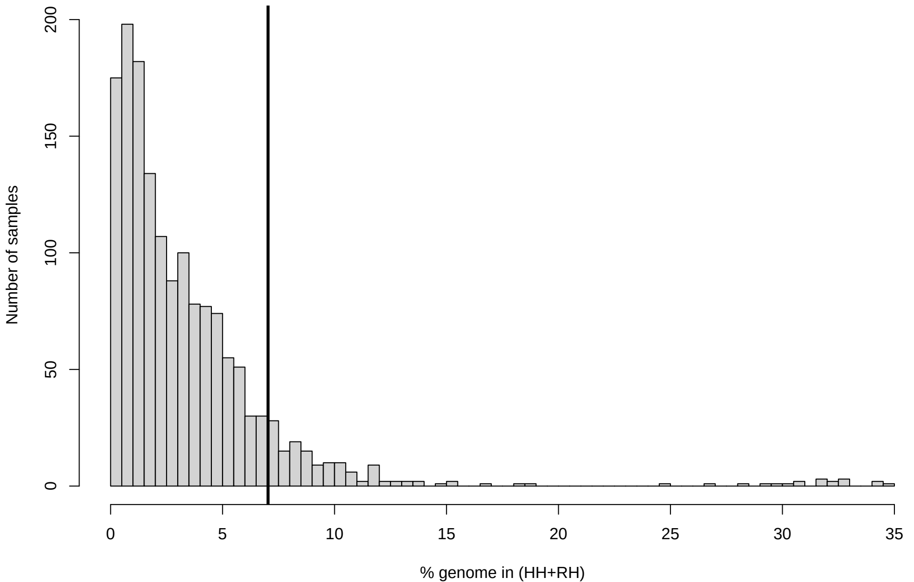
Observed donor % (HH+RH) vs expected BC2S3
