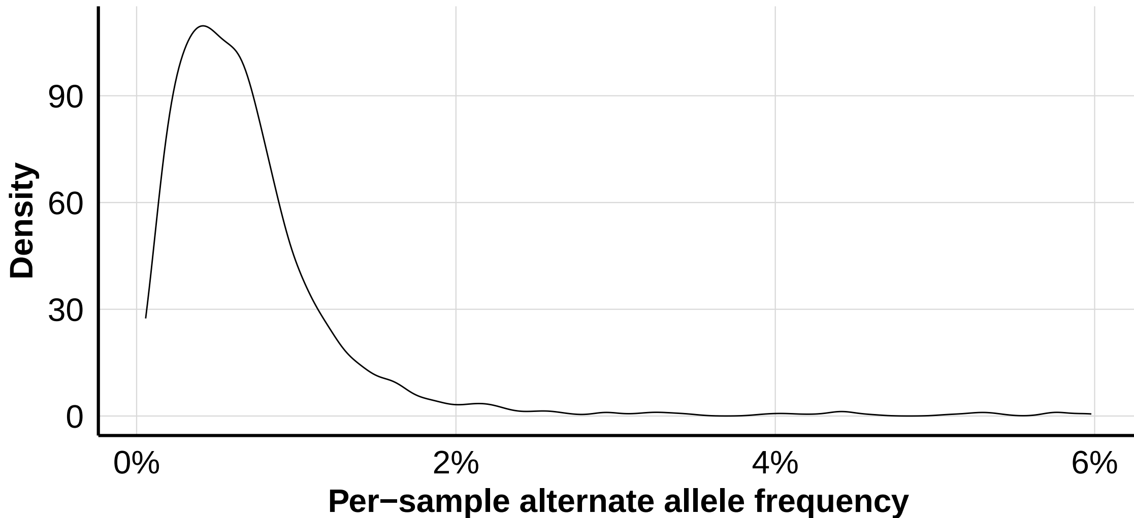
Per-sample alt allele frequency: Unfiltered
