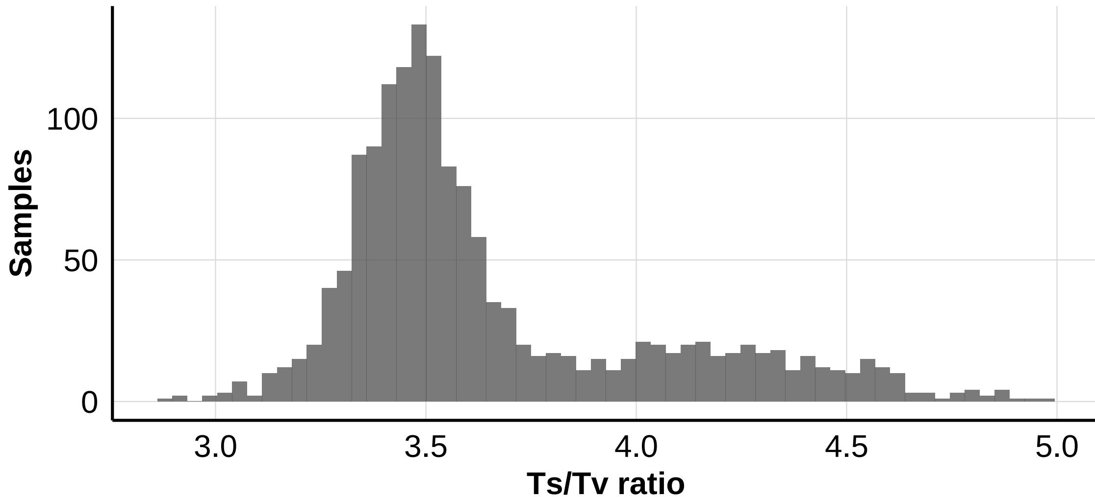
Ts/Tv: Unfiltered
