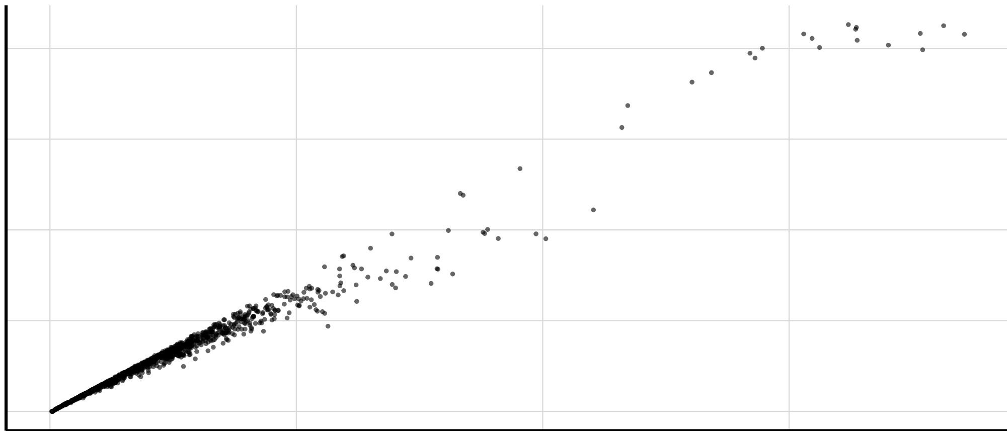
Hets vs alt burden: imputed
